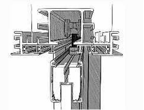
Sliding door "MODULAR RASO" Frame without cover-joint adaptable to standard counterframes Single door Mod. TransparentL_TRANSPARENT Collection
