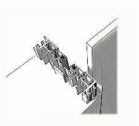
Sliding door "MODULAR RASO" Frame without cover-joint adaptable to standard counterframes Single door Mod. TransparentL_TRANSPARENT Collection
